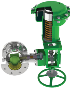
VTX70 Rotary Eccentric Plug General Service Control Valve
