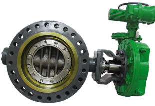
TVT80 Triple Offset Butterfly Valve
