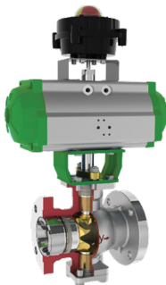
VTX90 V-Ball General Service Control Valve
